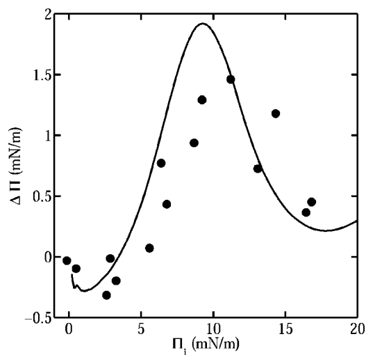
FIG. 3. Dependence of photo-induced surface pressure jump, \Delta\Pi = \Pi_i - \Pi_f , on the initial monolayer surface pressure in “dark,” \Pi_i (solid circles). The solid line represents the difference in the monolayer surface pressures for two different values of the subphase pH , 7.0 and 8.3, calculated from Fig. 1(a).
