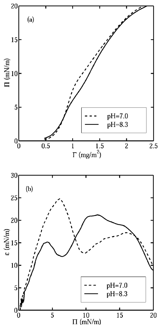
FIG. 1. (a) Surface pressure–surface concentration isotherms of \beta -casein monolayer at pH=7.0 (dashed line) and pH=8.3 (solid line). The subphase pH was adjusted by 100 mM phosphate buffer. (b) Static dilational modulus, \epsilon , as a function of the surface pressure, \Pi , as calculated from (a).
