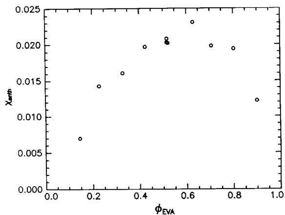
Figure 4 Values of the interaction parameter calculated from enthalpies of mixing ( \chi_{\text{enth}} ) as a function of the volume fraction of EVA
