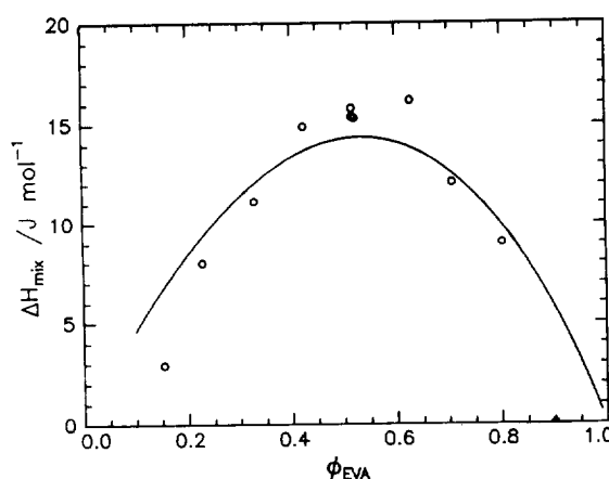
Figure 9 Fit (solid line) of equation (16) to enthalpy of mixing data as a function of EVA volume fraction. Fitting variables: \beta_{\text{H}} and \gamma
